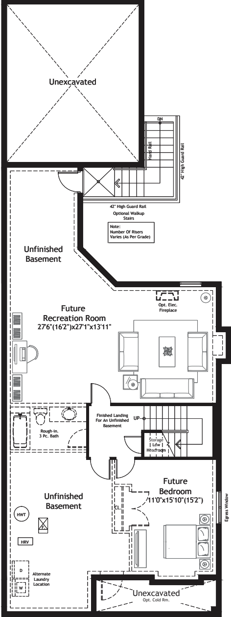
Basement - Elev. 'C' - 990 SQ. FT.
