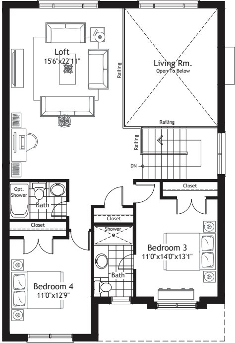
Opt. Loft Plan - Elev. 'C'
