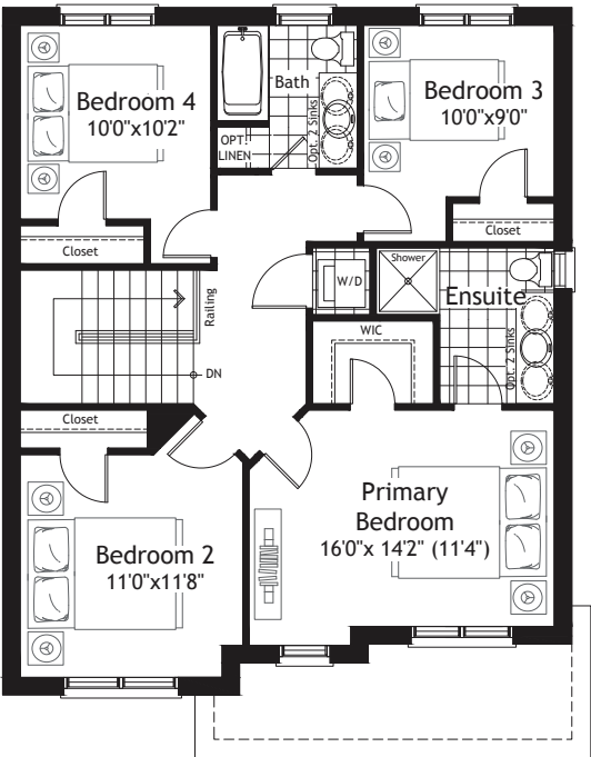
Alternative Second Floor 4 Bedrooms
