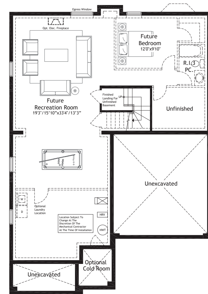
Basement Plan
