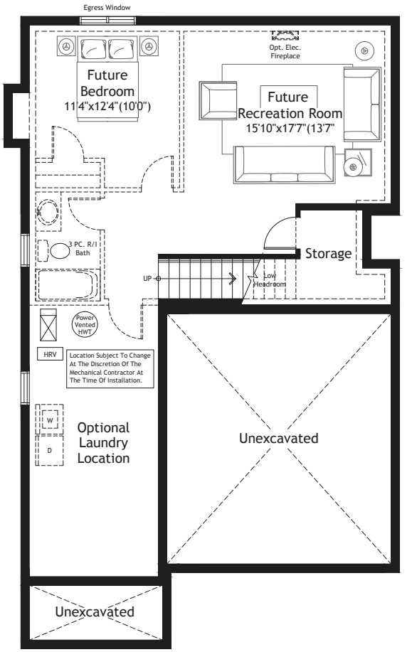
Basement
